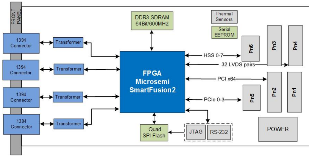
> V1142 PMC/XMC Block Diagram
