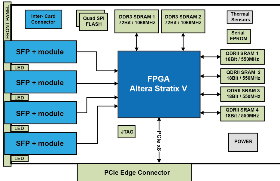
> V5031 Quad -Port PCI Express FPGA Card Block Diagram
